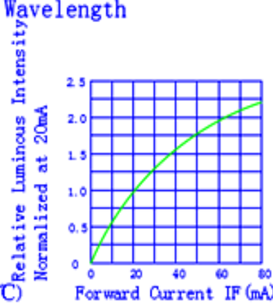
Fig.4 Relative Luminous Intensity vs. Forward Current
