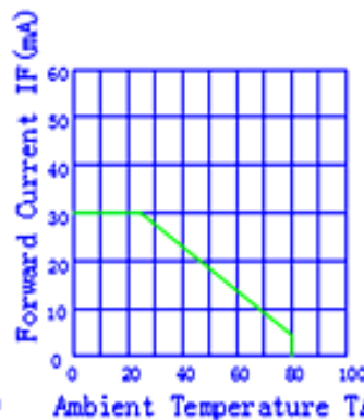
Fig.3 Forward Current vs. derating Curve
